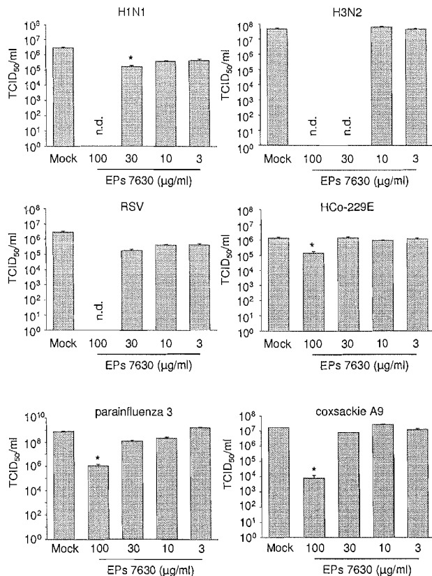
Fig. 1. Influence of EPs® 7630 on infectious virus titres indicated as 50% tissue culture infectious dose (TCID 50 /ml). EPs® 7630 was continuously present in cell culture media beginning with a 1 h pre-incubation period. Cells were infected with the respective viruses in the absence (Mock) or presence of EPs® 7630 at the following MOIs: influenza A virus H1N1, 0.005 (titres were determined 24 h post infection, cell line MDCK); influenza A virus H3N2, 0.005 (24 h, MDCK); coxsackie virus A9 (coxsackie A9), MOI 0.005 (24 h, human foreskin fibroblasts); parainfluenza virus type 3 (parainfluenza 3), 0.01 (72 h, LLC-MK2); respiratory syncytial virus (RSV), 0.01 (72 h, Vero); human coronavirus strain 229E (HCoV-229E), 0.01 (72 h, Caco-2). * P < 0.05 relative to Mock (as determined by ANOVA with subsequent Student-Newman-Keuls test); n.d. = not detectable.
